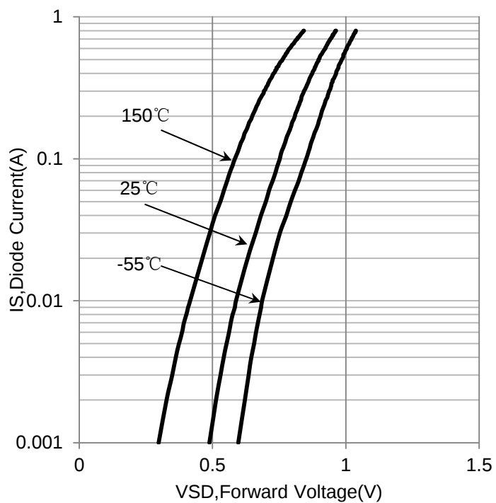
Body Diode Forward Voltage
